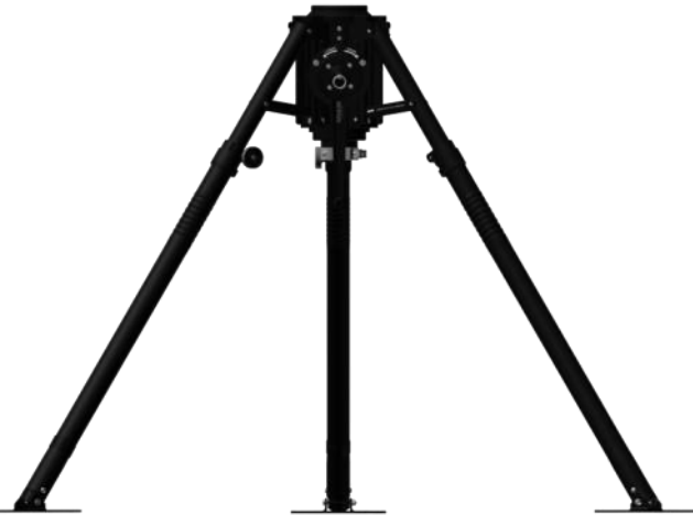
Qty: (1) Tripod with Bolted Lift Winch P/N: BSM2-K-T200-LFT-000 35.0 lbs / 15.2 kg
